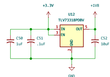
1.8V Power Supply
