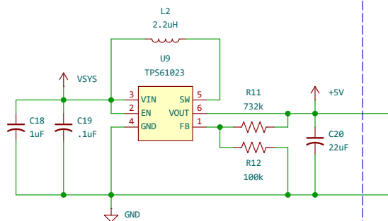
5V Power Supply
