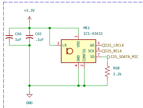
MEMS Microphone (I2S)
