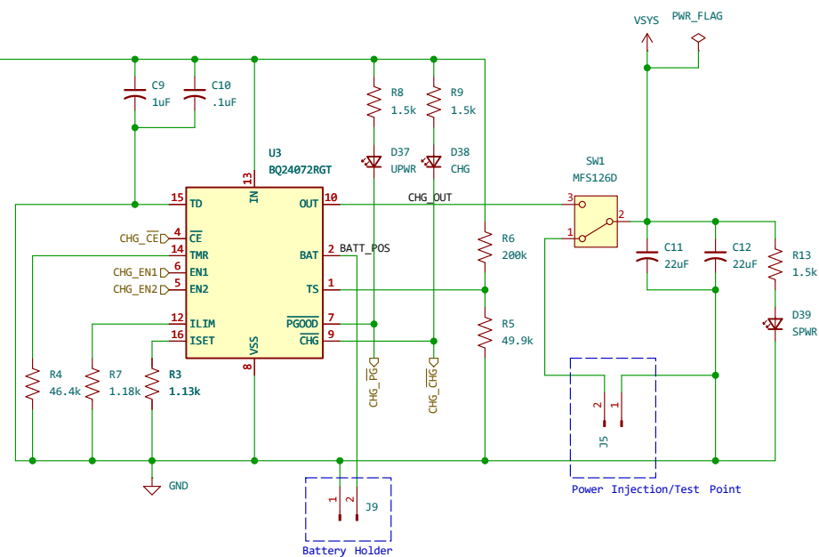
Battery Charger / Power Path
