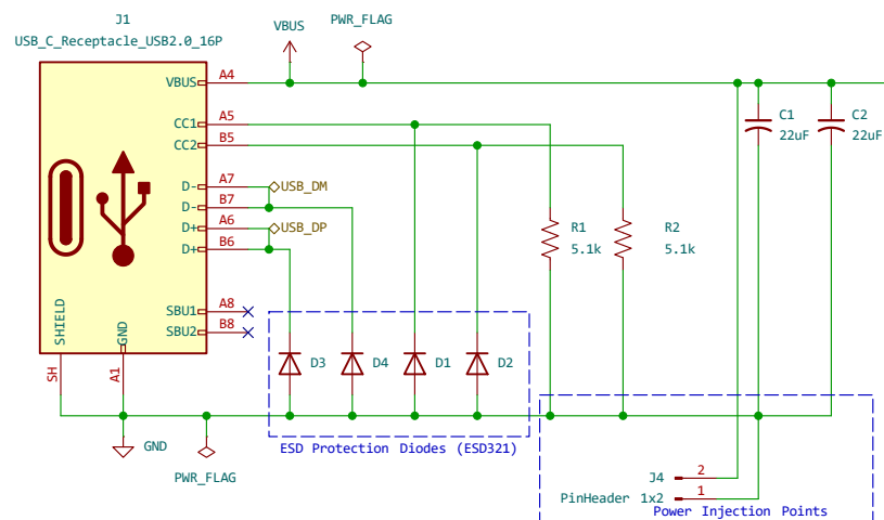
USB Connector
