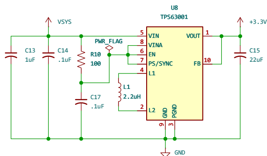
3.3V Power Supply
